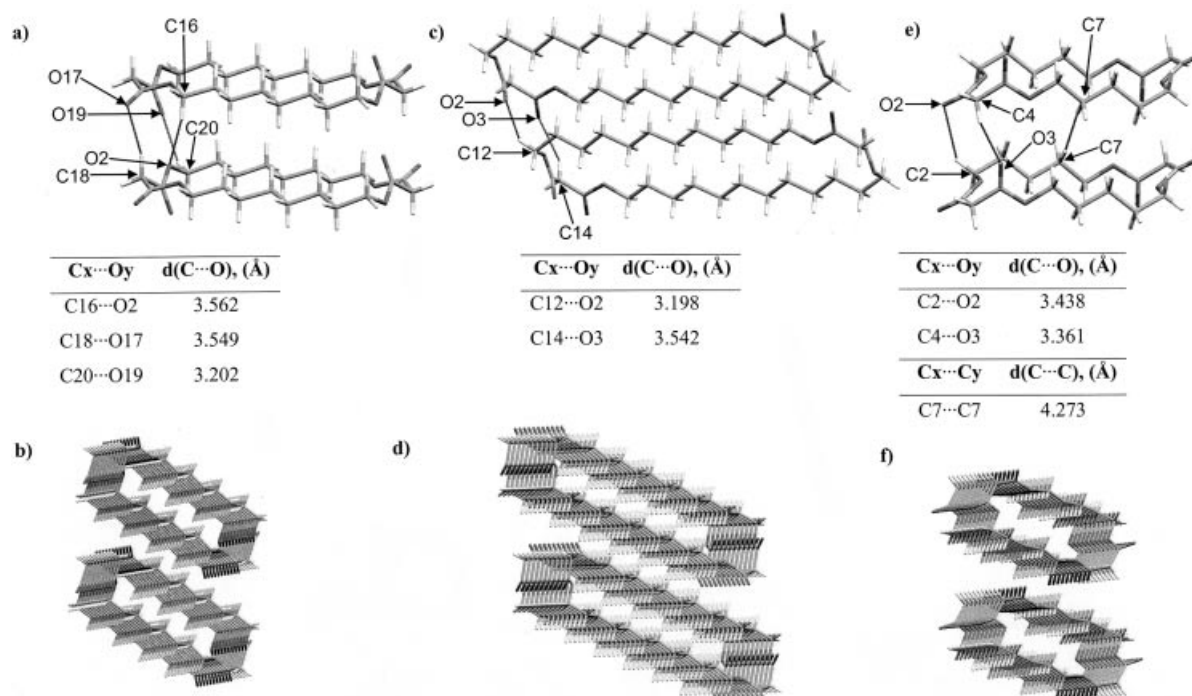
Figure 3. Columnar arrangement of 10b (left), [13] 12b (center), [13] and 9b (right) in single crystals: a) Intermolecular C–H...O hydrogen bonds between neighbouring molecules of 10b in the stacks and measured Cx...Oy distances. b) Columnar structure of 10b . c) Intermolecular C–H...O hydrogen bonds between neighboring molecules of 12b and measured Cx...Oy distances. d) Columnar structure of 12b . e) Intermolecular C–H...O hydrogen bonds and C–H...H–C interactions between neighbouring molecules of 9b and measured Cx...Oy and Cx...Cy distances. f) Columnar structure of 9b .
