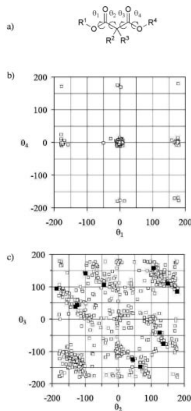
Figure 7. a) General graphical representation of the geometrical parameters used for the CSD search. b) Scatterplot correlating the pair of torsion angles ( \theta_1, \theta_4 ). c) Scatterplot correlating the pair of torsion angles ( \theta_2, \theta_3 ) (filled squares represent parameters for molecules described in this article).
