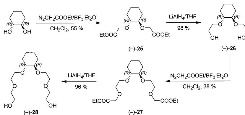
Scheme 3. Synthesis of the optically active diols (–)-26 and (–)-28.
