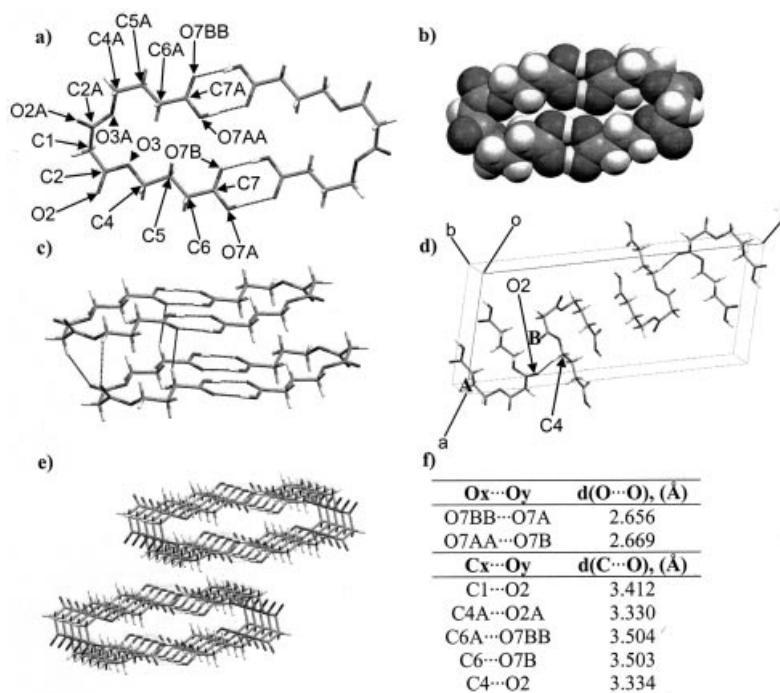
Figure 6. Molecular structure and columnar arrangement of 29 in the crystal. a) X-ray crystal structure of 29 and numbering of atoms. b) Space-filling representation of the supramolecular dimer. c) Intermolecular C-H...O hydrogen bonds between dimers of the same stack. d) Unit cell representation with the C-H...O hydrogen bond between molecules A and B. e) Columnar structure formed by the dimers. f) Measured distances for hydrogen bonds O-H...O and C-H...O.
