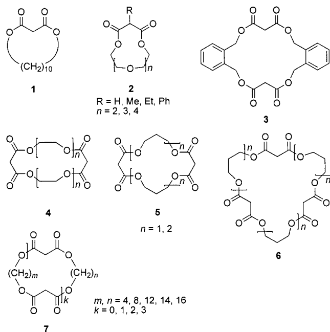
Scheme 1. Cyclic oligomalonate esters reported in the literature.
