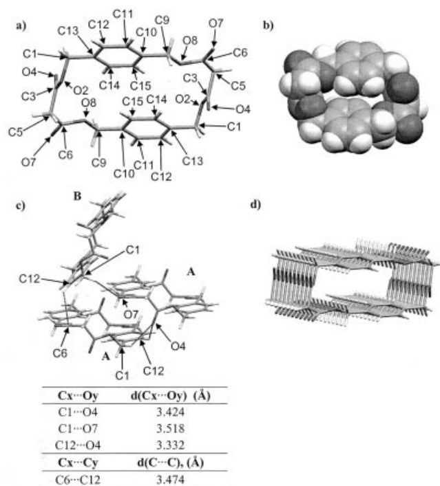
Figure 4. Molecular structure and columnar arrangement of 18b . a) X-ray crystal structure of 18b with numbering of atoms. b) Space-filling representation of the molecular structure. c) Alignment of the two molecules A and B with different structures found in the unit cell, intermolecular C–H \cdots O hydrogen bonds and C–H \cdots C=O interaction between molecules of the same kind in a columnar alignment and between molecules of a different kind, and measured C \cdots O and C \cdots C distances. d) Columnar structure formed by molecule A.
