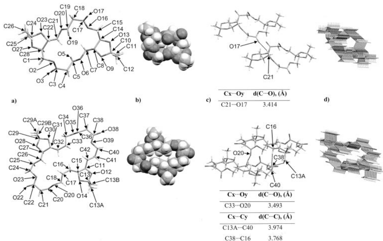
Figure 5. Molecular structure and columnar arrangement of (+)- 23b (top) and (+)- 24b (bottom). a) X-ray crystal structures with numbering of atoms. b) Space-filling representation of the molecular structures. c) C-H...O hydrogen bonds and C-H...H-C interactions between molecules in a columnar alignment and their measured distances. d) Columnar structures showing the channels formed in the crystal.
