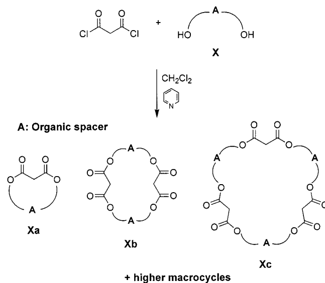
Scheme 2. Synthesis of macrocyclic oligomaltonates by condensation of malonyl dichloride with diols.
