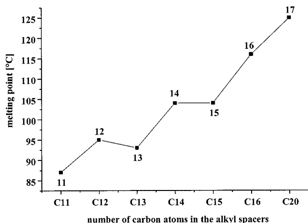
Figure 2. Diagram of the melting points of the cyclo[2]alkylmalonates vs. the number of carbon atoms in the alkyl spacers.
